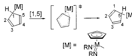
Scheme 2. [1,2]-metallotropic migration as [1,5]-sigmatropic rearrangement
