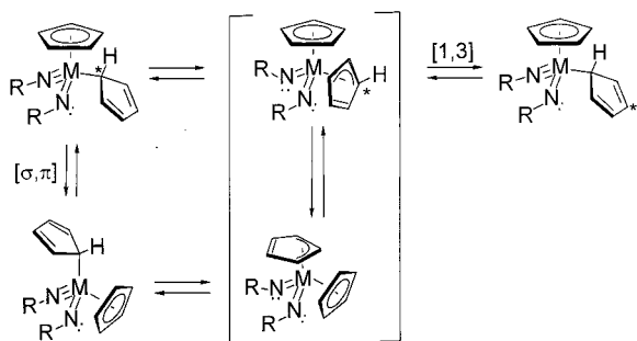
Scheme 1. Hapticity change and mechanistic proposal of a metallotropic rearrangement via allyl intermediates in complexes of the type [\eta^5\text{-C}_5\text{H}_5]\text{M}(\text{NR})_2(\eta^1\text{-C}_5\text{H}_5) ( M = Mo, W)
