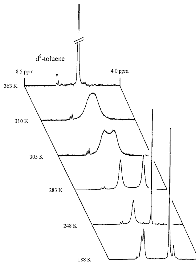
Figure 2. Variable temperature proton NMR spectra of [(\eta^5\text{-C}_5\text{H}_5)\text{Mo}(\text{N}t\text{Bu})_2(\eta^1\text{-C}_5\text{H}_5)] ( 2a ) in [\text{D}_8]\text{toluene} showing the \text{C}_5\text{H}_5 region from \delta = 4.00 to 8.50
